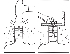
Drop-In Anchor Removable
